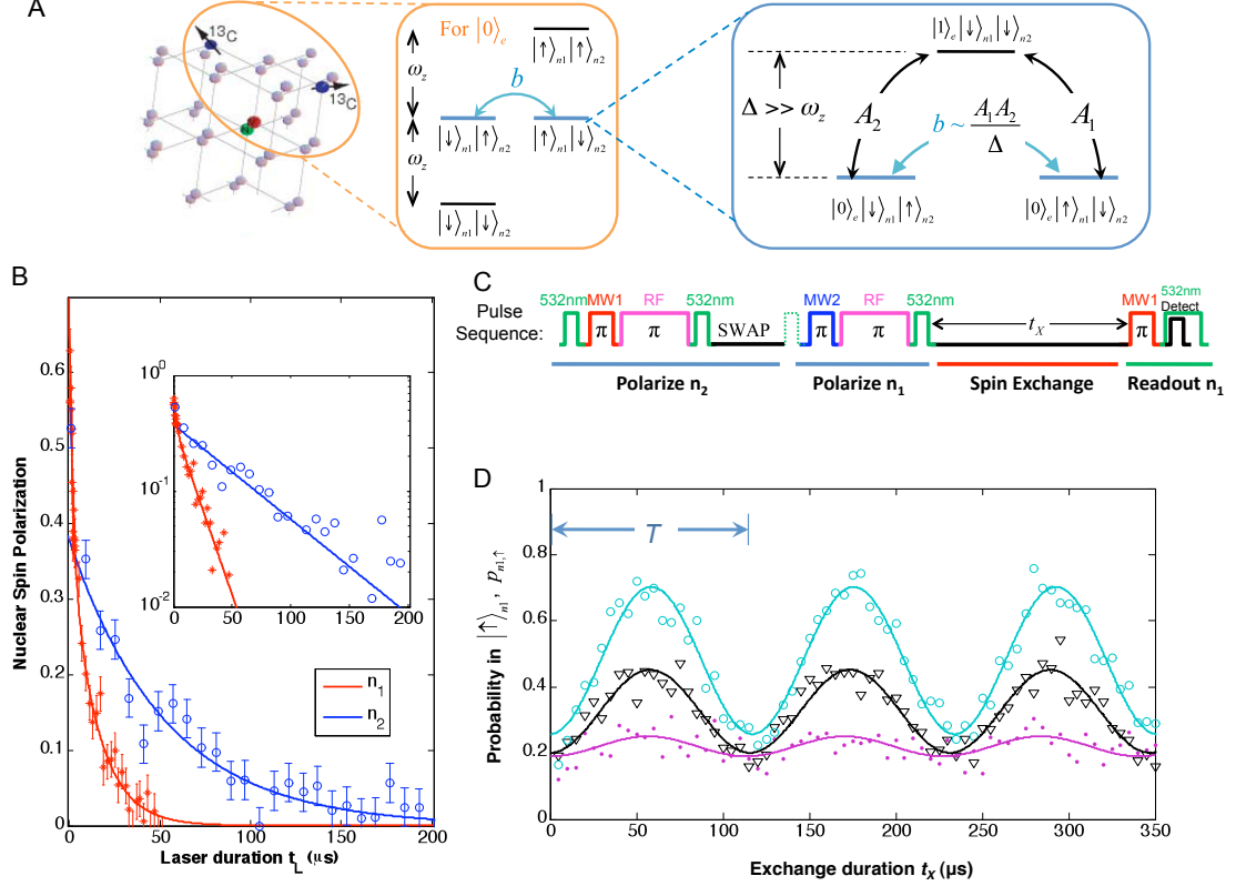
Figure A.3: | Coherence and control of two nuclear spins. (A) The coupled spin system formed by the NV electronic spin ( e ) and two proximal ^{13}\text{C} nuclear spins ( n_1 and n_2 ). Middle inset: Energy levels for spins n_1 and n_2 when spin e is in the |0\rangle_e state. Right inset: Schematic of flip-flop between spins n_1 and n_2 , which is electron-mediated by the second-order hopping via |1\rangle_e |\downarrow\rangle_{n_1} |\downarrow\rangle_{n_2} . (B) Measured depolarization of spins n_1 and n_2 under optical illumination. For the duration of optical illumination t_L longer than 1 \mu\text{s} , the polarizations for spins n_1 and n_2 decay exponentially with characteristic times \tau_{n_1} = 13 ( 1 ) \mu\text{s} and \tau_{n_2} = 53 ( 5 ) \mu\text{s} , respectively. For t_L less than 1 \mu\text{s} , the decay is slightly faster, which is likely associated with dynamics of the spin-fluctuator model that describe optically induced depolarization of single nuclei [67]. These decay times are much longer than the optical readout/pump time of the electronic spin (about 350 ns). Inset: Log-linear plot. (C) Operations and pulse sequence to probe dynamics between spins n_1 and n_2 . (D) Measured spin flip-flop dynamics between spins n_1 and n_2 . For three different preparations of the initial state ( |\downarrow\rangle_{n_1} |\uparrow\rangle_{n_2} (cyan), |\downarrow\rangle_{n_1} and n_2 in thermal state (black), and |\downarrow\rangle_{n_1} |\downarrow\rangle_{n_2} (purple)), the observed population, p_{n_1, \uparrow}(t) , oscillates with the same period T = 117 ( 1 ) \mu\text{s} . These observations verify the theoretical prediction, with flip-flop coupling strength b = 4.27 ( 3 ) kHz.
