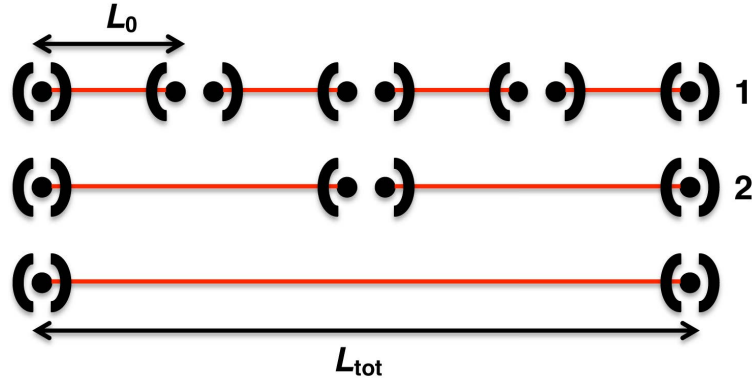
Figure 5.1: The general architecture of a quantum repeater. The total distance, over which entanglement should be distributed, is divided into elementary links of length L_0 connected by repeater stations pictured as cavities containing single emitters. After creating entanglement in the elementary links, the entanglement is swapped to larger distances by combining the elementary links. The numbers to the right in the figure refers to the swap level of the repeater. In the first swap level, the four elementary links are connected pairwise to make two longer links. In the second swap levels these two links are connected to create entanglement over the total distance. The total number of swap levels is thus 2 for this depicted setup.
