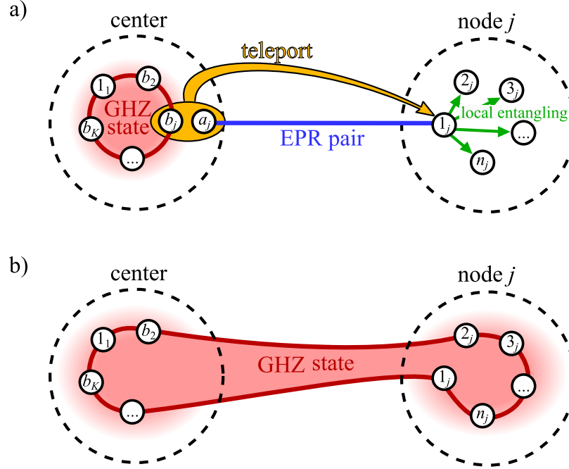
Figure 7.2: Entangled state preparation between distant nodes. a) The center node ( j = 1 ) initiates the initialization sequence by preparing a local GHZ state across the qubits \{b_j\}_{j=2}^K and 1_1 , as well as (K - 1) EPR pairs on the qubit pairs \{(a_j, 1_j)\}_{j=2}^K . Quantum teleportation expands this GHZ state to the first qubit within each of the individual nodes. b) Originating from the teleported qubits, the nodes grow the GHZ state to involve all the desired local qubits by employing local entangling operations. The procedure results in a common GHZ states over all atoms of the nodes.
