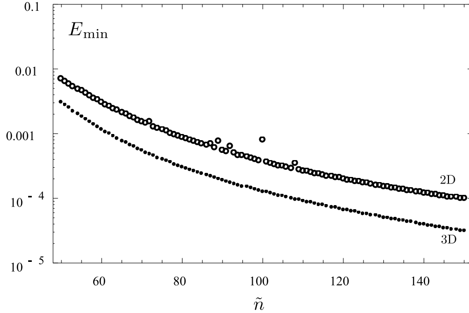
Figure G.3: The minimized error contribution of a single atom as a function of the principle quantum number of the Rydberg levels \tilde{n} , for the 2D and 3D setup.
