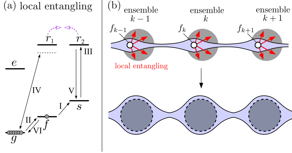
Figure 8.3: Local GHZ creation. (a) Conditional, local GHZ state generation: Any excitation in level s prevents the dressing of g with r_1 , which, otherwise introduces a \pi phase shift on g . With the conjugation of \pi/2 pulses II and VI, this results in a transfer from g to f conditioned on the population of s . (b) The local entangling operation extends the GHZ state from the f spin-wave to all atoms. As a result, every atom in the network gets entangled.
