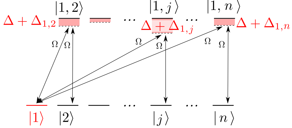
Figure G.1: Different single excitation states ( |j\rangle = \sigma_j^\dagger |gg\dots g\rangle , j = 1, 2, \dots, n ) are resonantly coupled to each other through a Raman-transition via double excited states ( |j, k\rangle = \sigma_j^\dagger \sigma_k^\dagger |gg\dots g\rangle , j < k ). The effective coupling strengths depend on the detuning of the intermediate level, and results in an inhomogeneous broadening. (The figure shows only the double excited states that couple to |1\rangle .)
