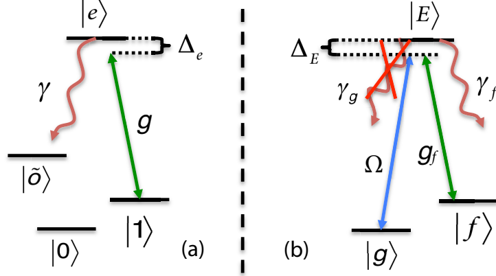
Figure 4.1: (a) Level structure of the qubit atoms. Only state |1\rangle couples to the cavity and we assume that the excited level decays to some level |\tilde{o}\rangle , possible identical to |f\rangle or |0\rangle . (b) Level structure of the auxiliary atom and the transitions driven by the weak laser ( \Omega ) and the cavity ( g_f ). We assume that |E\rangle \leftrightarrow |f\rangle is a closed transition, i.e. \gamma_g = 0 .
