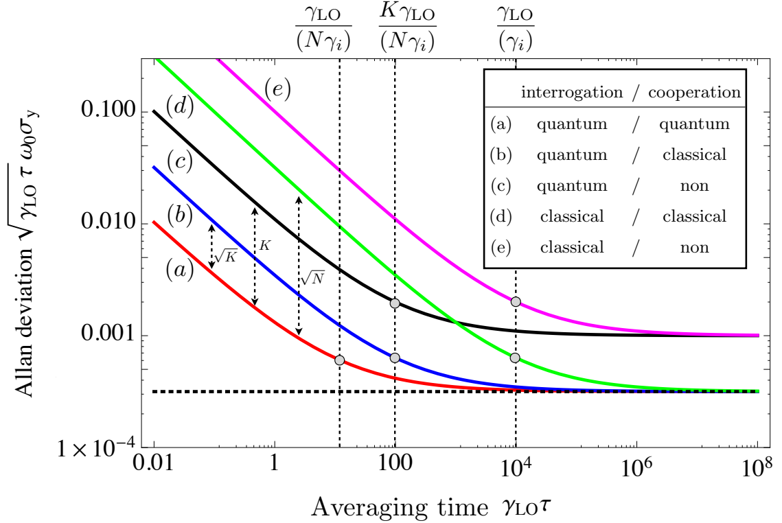
Figure 7.3: Performance of different operation schemes. Comparison of the achievable (rescaled) Allan deviation \sqrt{\gamma_{\text{LO}} \tau \omega_0 \sigma_y} using clock networks of different types and degrees of cooperation. (a) the proposed protocol realizing quantum interrogation and cooperation, (b) quantum interrogation and classical cooperation, (c) quantum interrogation and no cooperation, (d) classical interrogation and classical cooperation, (e) classical interrogation and no cooperation (cf. text). The dotted base line represents the fundamental bound arising from the finite width of the clock atoms transition [compare Eq. 7.4]. This optimal stability can be attained only via cooperation between the nodes. The quantum clock network (a) represents the optimal form of cooperation, and reaches this boundary faster than any other operational mode. Parameters are N = 1000 , K = 10 , \gamma_i = 10^{-4} \gamma_{\text{LO}} .
