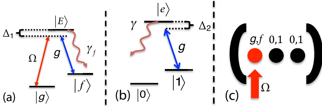
Figure 5.3: Schematics of the heralded CZ gate [26]. (a) is the level structure of the auxiliary atom, (b) is the level structure of the qubit atoms and (c) shows the cavity containing the auxiliary atom and the two qubit atoms. Assuming that |E\rangle only decays to |f\rangle by e.g. driving the transition |g\rangle \rightarrow |E\rangle with a two photon process, any spontaneous emission or cavity decay will change the state of the auxiliary atom from the initial state |g\rangle to |f\rangle . The gate is thus conditioned on measuring the auxiliary atom in state |g\rangle at the end of the gate.
