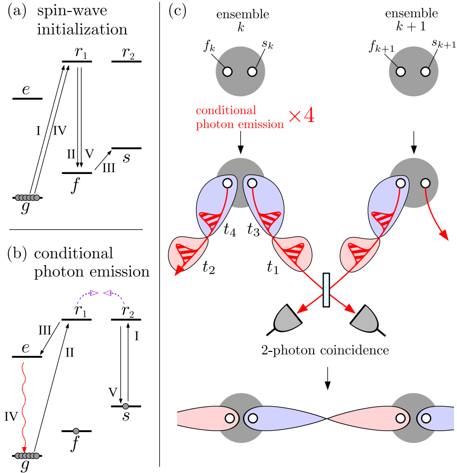
Figure 8.1: Steps to generate pairwise entanglement. (a) Pulse sequence used to initialize the spin-waves f and s in an ensemble. (b) Pulse sequence inducing a conditional photon emission, the emitted photon becomes entangled with the spin state s . (c) In three steps, neighboring ensembles generate pairwise entanglement between their collective excitations. First, they induce 0+1 superpositions of the two independent spin waves, f^\dagger and s^\dagger . Then applying the conditional photon emission sequence four times, they emit four pulses, containing two photons total. Each pair of photons is correlated with a unique spin state. Finally, photons are measured with a linear optics setup, and 2-photon coincidences indicate the creation of entanglement between neighboring ensembles.
