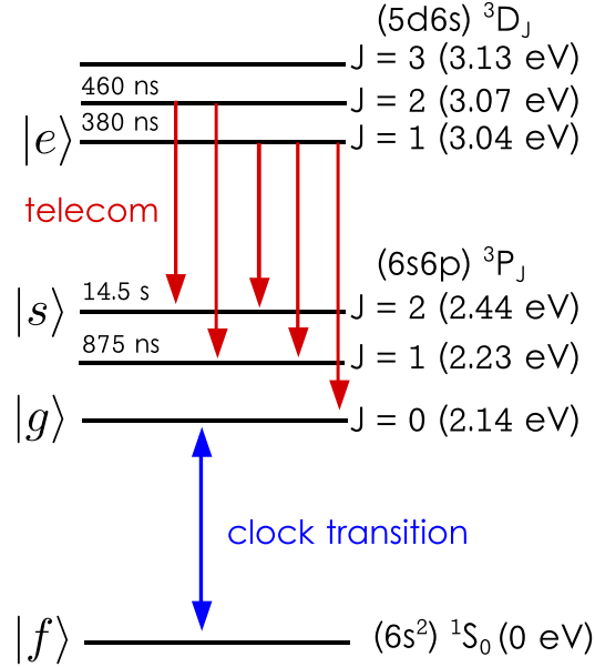
Figure 8.4: Implementation of our protocol in the lower level of neutral Yb. We assign the roles of g and f to the clock levels, the role of s to the metastable J = 2 level of 6s6p , and the role of e to the J = 1 level of the excited state 5d6s , which spontaneously decays to all three levels of 6s6p state by emitting a telecom frequency photon.
