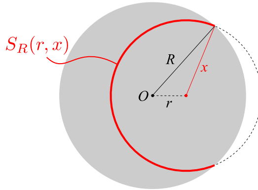
Figure G.7: The length of the circle segment of radius x lying inside the cloud of radius R , S_R(r, x) , is between 0 and 2\pi x for R - r < x < R + r , where r is the separation between the centers.
