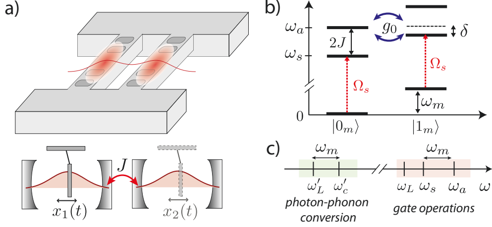
Figure 3.1: a) Setup of two tunnel-coupled OM crystal cavities (see Ref. [79, 42] for more details). b) Level diagram showing the lowest mechanical and optical excitations in a two mode OMS. Resonant coupling ( \delta = 0 ) occurs when the tunnel splitting 2J between the optical modes is comparable to the mechanical frequency \omega_m . c) Different sets of strongly and weakly coupled optical modes and control laser fields can be used for nonlinear interactions ( \omega_s, \omega_a, \omega_L ) and purely linear photon storage and retrieval operations ( \omega'_c, \omega'_L ).
