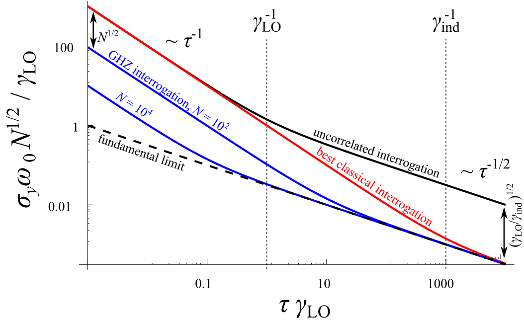
Figure 6.2: Allan deviation \sigma_y for different protocols as a function of averaging time \tau , normalized to the standard quantum limit, for \gamma_{LO}/\gamma_{ind} = 10^3 . The solid black line corresponds to the standard scheme using a single uncorrelated ensemble. It fails to reach the fundamental noise floor set by the atomic transition linewidth (cf. Eq. 6.5, broken line). A more sophisticated classical scheme which uses exponentially increasing Ramsey times in each cycle [183, 27] allows to extend the regime of linear scaling with 1/\tau up to the point where the bound (6.5) is met. In comparison, the proposed cascaded GHZ protocol (blue solid curves) enables an \sim N times faster convergence. For short averaging times the stability is enhanced by a factor \sqrt{N} as compared to classical protocols.
