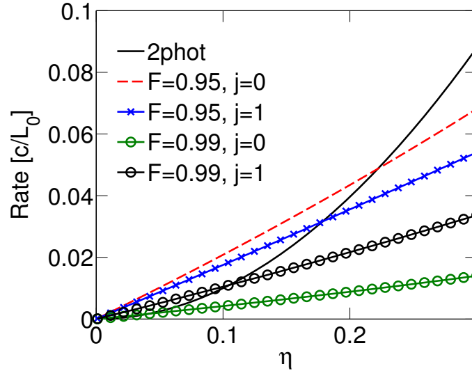
Figure 5.6: Rate of entanglement generation for the two-photon scheme and the single-photon scheme with target fidelity F \geq 0.95 and F \geq 0.99 both without purification ( j = 0 ) and with one round of purification ( j = 1 ). The rate is shown as a function of the total detection efficiency \eta . We have neglected dark counts and assumed that the CNOT gate is deterministic and have perfect fidelity. The rate has been calculated as described in App. D.4. Furthermore, we have assumed that each repeater station contains 4 qubits, which are either used for purification or to increase the rate of the entanglement generation.
