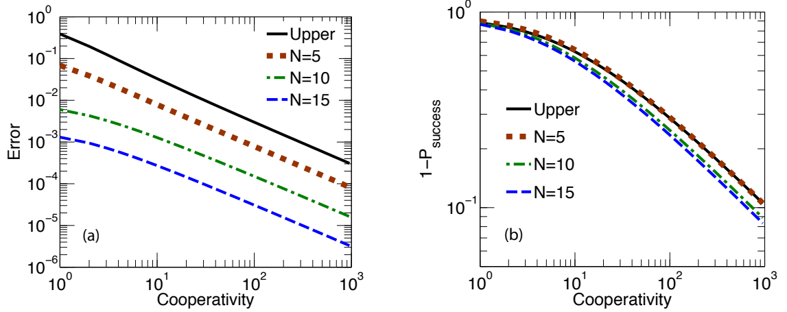
Figure C.2: (a) Gate error of the Toffoli for different initial states as a function of cooperativity. We have plotted the generic error for N = 5, 10 , and 15 and the upper bound of the error. Note that the generic error decreases as N increases. We have fixed \Delta such that \Gamma_0 = \Gamma_1 and have assumed that \alpha = \beta = 1 . (b) The failure probabilities 1 - P_{\text{success,up}} and 1 - P_{\text{success,gen}} as a function of cooperativity. 1 - P_{\text{success,gen}} is plotted for N = 5, 10, 15 . We have used the same assumptions as in (a). In general, the failure probability only have a weak dependence on N . Note that the line for 1 - P_{\text{success,gen}}, N = 5 coincides with 1 - P_{\text{success,up}} .
