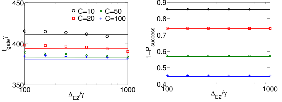
Figure C.6: Gate time (left) and failure probability (right) as a function of \Delta_{E2} for \gamma = \gamma_g = \gamma_f = 0.01\kappa , \Omega = \frac{\Delta_{E2}}{8C^{1/4}} , \Omega_{\text{MW}} = 4\gamma C^{1/4} , C = \{10, 20, 50, 100\} .
