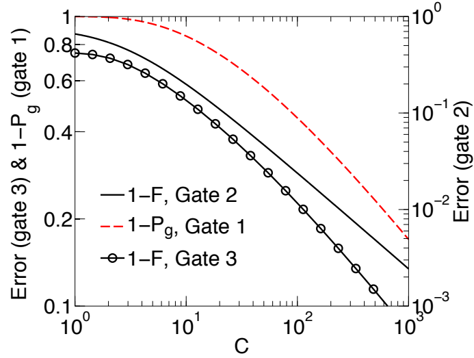
Figure 5.8: Characteristics of the three gates described in the text. The errors of gate 2 (black/solid line, right axis) and gate 3 (black/circled line, left axis) are shown as a function of the cooperativity. The error is defined as 1 - F where F is the fidelity of the gate. We have assumed \eta_d = 0.5 for the error of gate 2. Gate 1 has conditional fidelity \sim 1 but a finite failure probability 1 - P_g which is also shown as a function of cooperativity (red/dashed line, left axis).
