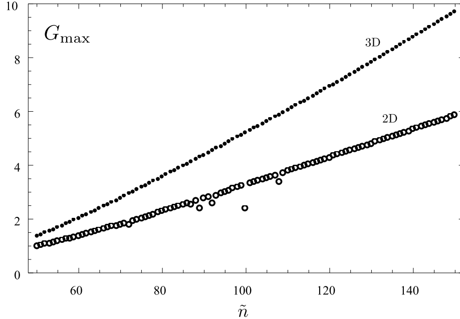
Figure G.6: Maximal gain over the non-entangled scheme provided by the optimal entangled clock network architecture as a function of principle quantum number of the Rydberg states \tilde{n} , for the 2D and 3D setup.
