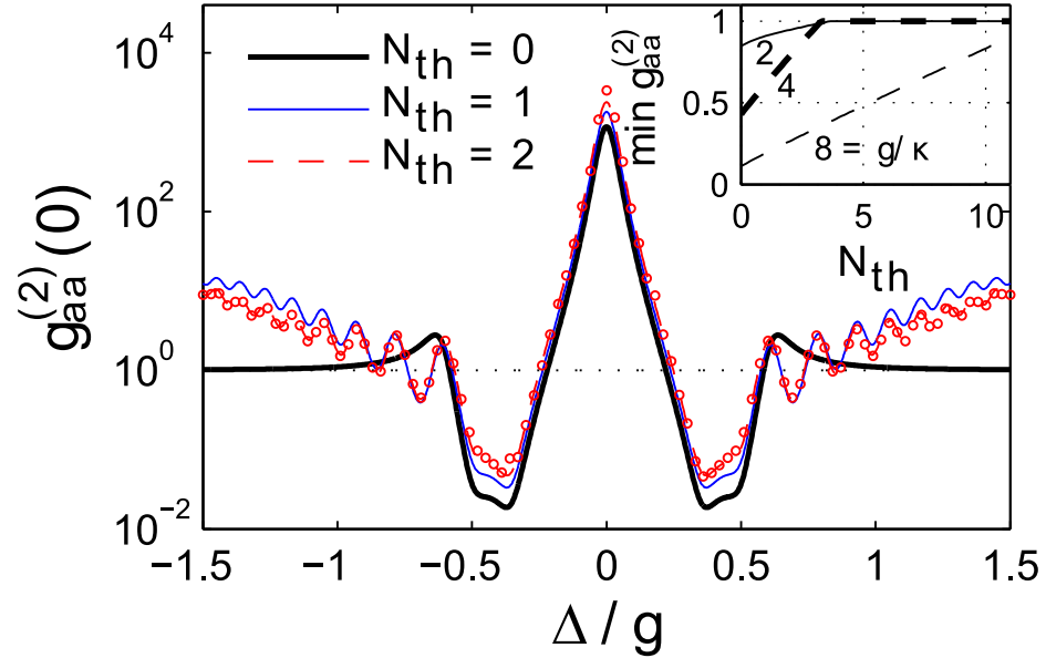
Figure 2.9: Driven mode correlation function g_{aa}^{(2)}(0) for thermal mechanical occupation N_{\text{th}} = 0, 1, 2 . Solid lines show the analytic calculation with \gamma \rightarrow 0 , and dots show the full numerical results for N_{\text{th}} = 2 only. The inset shows the minimal g_{aa}^{(2)}(0) as a function of N_{\text{th}} for several coupling strengths. Parameters are g/\kappa = 20 , and (for numerics) \gamma/\kappa = 10^{-3} .
