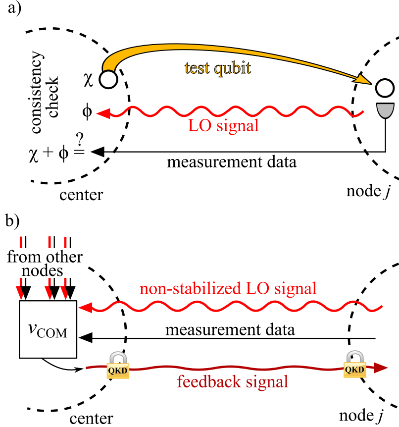
Figure 7.4: Schematics of security countermeasures. a) The center node can choose to test any node j by teleporting a disentangled qubit with a certain phase rotation. A properly operating node creates a local GHZ state [|0\rangle + e^{i\chi}|1\rangle]/\sqrt{2} from the sent qubit, measures the parity of the GHZ state, and sends it to the center. The measured parity holds information on the phase \phi' = \chi + \phi , where \phi is the accumulated phase of the LO at the node. The center verifies \phi by comparing it with the classically determined phase of the sent LO signal with respect to the COM signal. b) Eavesdropping can be prevented by prescribing that only the non-stabilized LO signals are sent through classical channels and encoding the radio frequency feedback signal with phase modulation according to a shared secret key.
