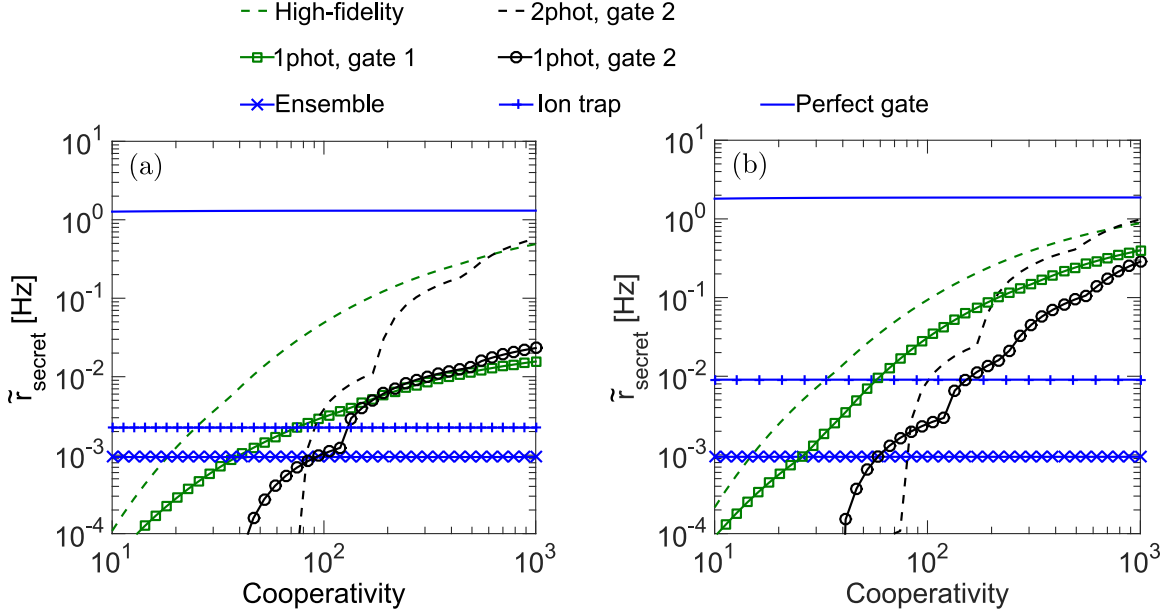
Figure 5.11: Normalized secret key rate per station ( \tilde{r}_{\text{secret}} ) as a function of the cooperativity ( C ) for the high-fidelity repeater and other repeaters assuming a distribution distance of 1000 km. (a) is for 2 qubits per repeater station while (b) is for 4 qubits per repeater station.
