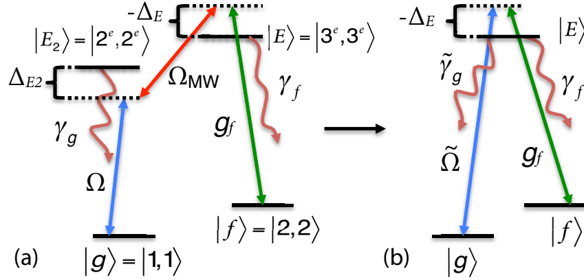
Figure 4.3: (a) Level structure of the auxiliary atom and the transitions driven by a weak laser ( \Omega ), a microwave field ( \Omega_{\text{MW}} ) and the cavity ( g_f ). We assume that |E\rangle \leftrightarrow |f\rangle is a closed transition and, for simplicity, we also assume that |E_2\rangle \leftrightarrow |g\rangle is a closed transition but this is not a necessity. Here |r^{(e)}, r^{(e)}\rangle with r = 1, 2, 3 refers to how the atom may be realized in the ( 5^2P_{3/2} ) states |F^{(e)} = r, m^{(e)} = r\rangle 5^2S_{1/2} of Rb 87 . (b) Effective three-level atom realized by mapping the two-photon drive to give an effective decay rate \tilde{\gamma}_g and an effective drive \tilde{\Omega} .
