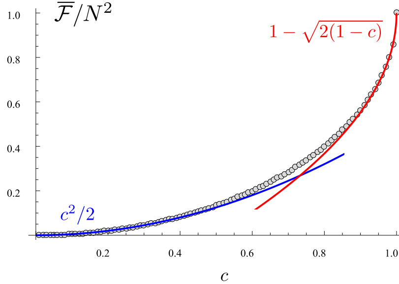
Figure G.4: Average Fisher information as a function of the contrast c (dots). It is well approximation by c^2/2 for c < 0.6 and by 1 - \sqrt{2(1-c)} for c > 0.8 (solid curves).
