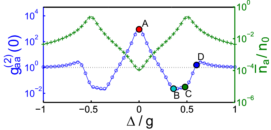
Figure 2.3: Normalized average photon number (green “+”) and photon-photon correlation function (blue “o”) for driven mode c_a as a function of laser detuning at zero temperature. Solid lines are calculated from analytic model (see Eqs. (2.19-2.24)) and points show full numerical calculation. The average photon number is normalized by n_0 = (\Omega/\kappa)^2 . ( g/\kappa = 20 and \gamma/\kappa = 0.2 )
