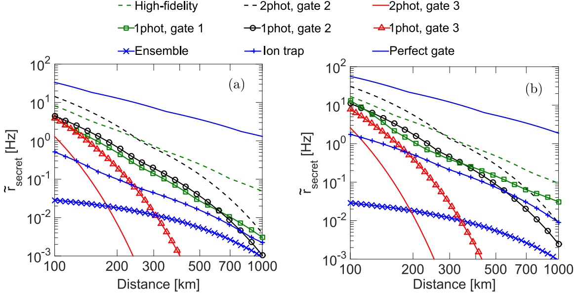
Figure 5.10: Normalized secret key rate per station ( \tilde{r}_{\text{secret}} ) as a function of the distribution distance (Distance) for the high-fidelity repeater and other cavity-based repeaters assuming a cooperativity of C = 100 . (a) is for 2 qubits per repeater station while (b) is for 4 qubits per repeater station. The other cavity-based repeaters are labelled as, e.g., “1photon, gate 2”, which indicates that it is a repeater based on the single-photon detection scheme and gate 2. The rate of an ensemble-based repeater (“Ensemble”) is also shown [193]. For simplicity, we have assumed a fixed number of four swap levels in the ensemble-based repeater even though a smaller number of swap levels might increase the rate for small distances ( \lesssim 400 km). Finally, we have plotted the rate of an ion trap repeater scheme (“Ion trap”) with a collection efficiency of 10% and gate fidelity of 99.3% and the ultimate rate obtainable with perfect deterministic gates and perfect entanglement generation with the two-photon scheme (“Perfect gate”) for comparison. For the ion trap repeater we have plotted the highest rate obtainable with either the one-photon or two-photon scheme.
