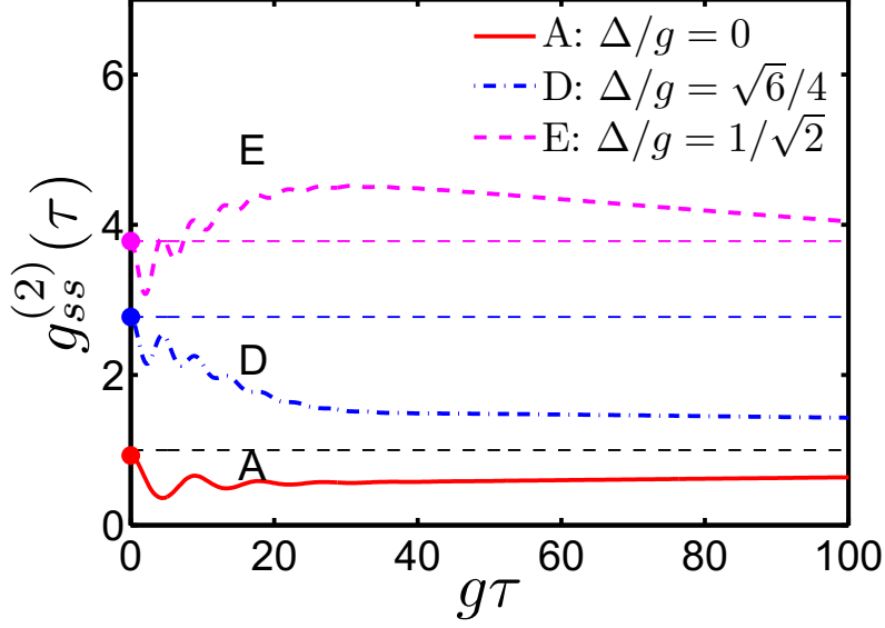
Figure 2.12: Finite time delay intensity correlation function g_{ss}^{(2)}(\tau) for detunings \Delta/g = 0 (A), \sqrt{6}/4 (D) and \frac{1}{\sqrt{2}} (E). Thin dashed lines indicate the classical bounds (see Eq. 2.37). Labels A, D, E correspond to the same detunings marked in Fig. 2.3 and Fig. 2.11. Parameters are g/\kappa = 8 , and \gamma/\kappa = 0.02 .
