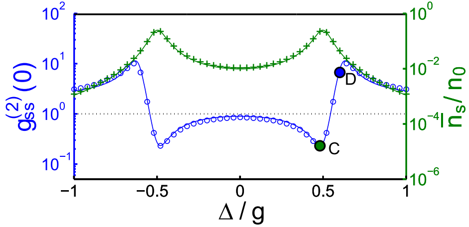
Figure 2.4: Normalized average photon number (green “+”) and photon-photon correlation function (blue “o”) for the undriven mode c_s as a function of laser detuning at zero temperature. Solid lines are calculated from analytic model (see Eqs. (2.19-2.24)) and points show full numerical calculation. The average photon number is normalized by n_0 = (\Omega/\kappa)^2 . ( g/\kappa = 20 and \gamma/\kappa = 0.2 )
