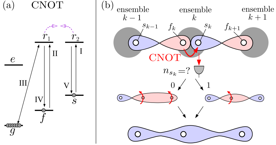
Figure 8.2: Connecting links into non-local GHZ state. (a) CNOT gate between the two excitations f and s : If level s is occupied, then the coherent (de)excitation of the f level is blocked by the Rydberg blockade between the r_1 and r_2 intermediate levels, otherwise it succeeds. (b) Connecting two entanglement links. The local CNOT and measurement operations on ensemble k entangle the two, initially independent, parts of the system: s_{k-1}, f_k and s_k, f_{k+1} . Depending on the outcome of the measurement, either only f_k , or the entire right hand side needs to be flipped, in order to arrive to the proper GHZ state.
