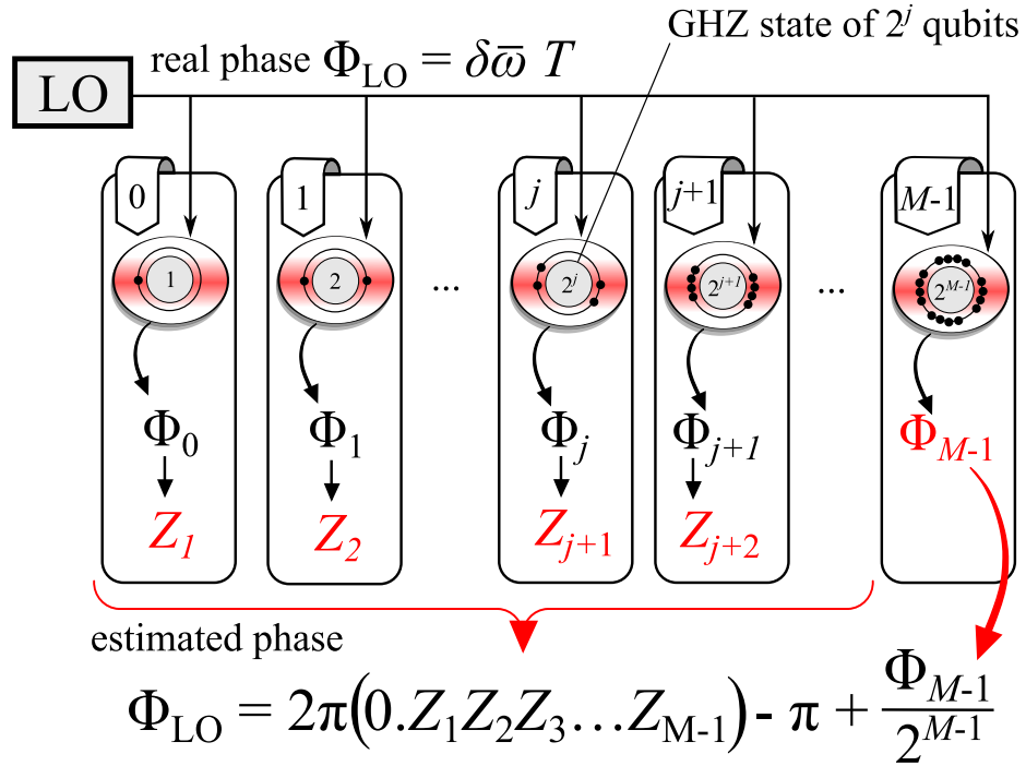
Figure 6.1: The proposed clock operation scheme employs M different groups of clock atoms prepared in correlated states of varying size to interrogate the relative phase \Phi_{\text{LO}} of the LO field. A single group j contains n_0 independent instances of GHZ-like states, each entangling 2^j qubits, and therefore accumulating a phase \Phi_j = 2^j \Phi_{\text{LO}} \bmod [-\pi, \pi] during a single cycle. Each group is then used to measure this phase, which gives a direct estimate on the digit Z_{j+1} in a binary representation of the LO phase (\Phi_{\text{LO}} + \pi)/2\pi = (0.Z_1Z_2Z_3\dots) , subsequently used to feedback the LO frequency.
