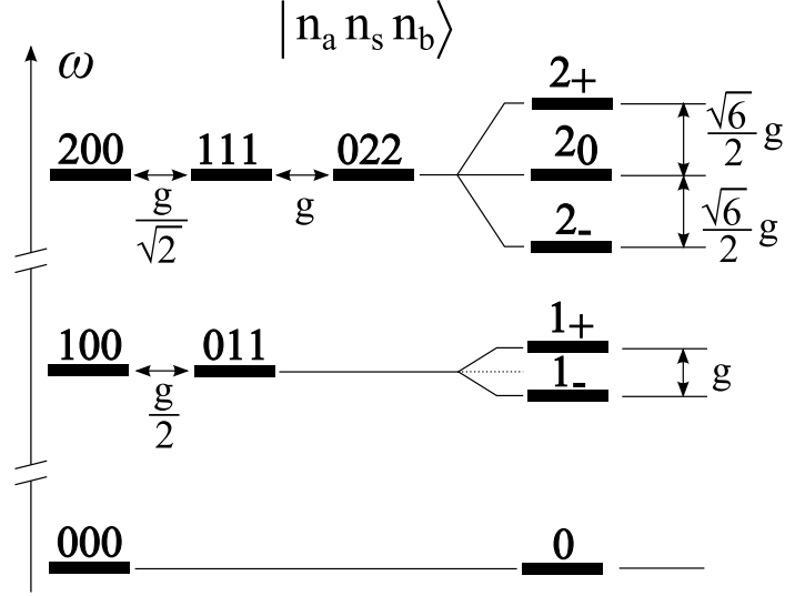
Figure 2.2: Level diagram showing the relevant zero-, one- and two-photon states at zero temperature and under the three-mode resonance condition \omega_s - \omega_a = \omega_m . States are labeled by |n_a n_s n_b\rangle denoting the number n_a ( n_s ) of antisymmetric (symmetric) photons and the number of phonons n_b . The optomechanical coupling g splits the degeneracy of states |n_a n_s n_b\rangle and |n_a - 1, n_s + 1, n_b + 1\rangle .
