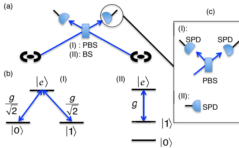
Figure 5.2: Entanglement generation in the elementary links where emission from two cavities are combined on a beam splitter. (a) shows the basic setup, (b) shows the level structure of the emitters and (c) shows the detection setup. (I) refers to the two-photon detection scheme and (II) refers to the single-photon detection scheme. Both schemes use a central station with either (I) three polarizing beam splitters (PBS) and four single-photon detectors or (II) a single balanced beam splitter (BS) and two single-photon detectors. g denotes the cavity coupling. For the two-photon scheme the levels |0\rangle and |1\rangle are assumed to have equal coupling of g/\sqrt{2} to the excited state |e\rangle .
