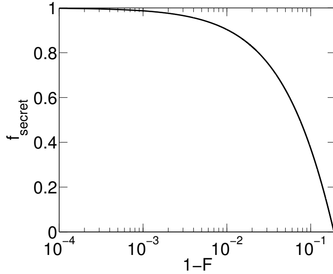
Figure 5.4: Secret key fraction ( f_{\text{secret}} ) as a function of the infidelity, 1 - F , of the final entangled pair. For 1 - F \gtrsim 19\% it is no longer possible to extract a secret key from the raw keys.
