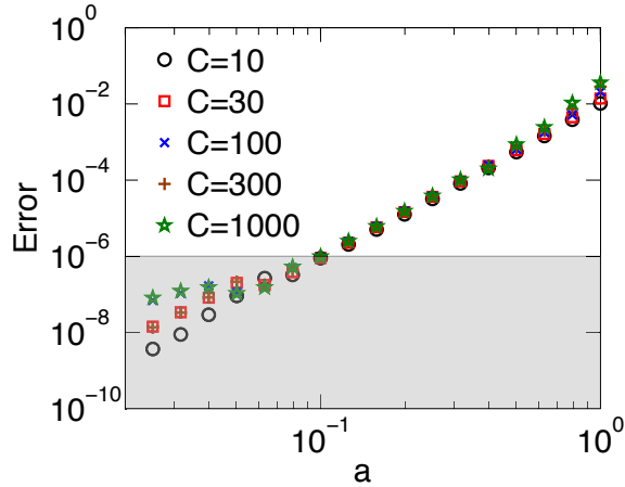
Figure C.5: Conditional infidelity of the gate as a function of the driving strength ( a ) for \gamma/\kappa = 0.01 , \gamma_g = 0 , and C \in \{10, 30, 100, 300, 1000\} . The shaded region (at \sim 10^{-6} ) shows the limit of numerical accuracy. The driving strength was assumed to be \Omega = a\gamma\sqrt{C} .
