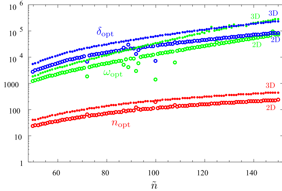
Figure G.2: The dressing fields optimal Rabi frequency \omega = \Omega/\gamma , detuning \delta = \Delta/\gamma and the optimal number of atoms in a single clock n is plotted as a function of the principle quantum number of the Rydberg levels \tilde{n} , for the 2D and 3D setup.
