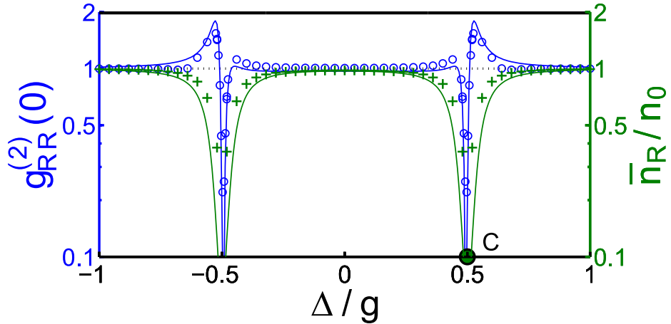
Figure 2.5: Normalized average photon number (green “+”) and photon-photon correlation function (blue “o”) for the reflected field c_R , as a function of laser detuning at zero temperature. Solid lines are calculated from analytic model (see Eqs. (2.19-2.24)) and points show full numerical calculation. The average photon number is normalized by n_0 = (\Omega/\kappa)^2 . The small discrepancy between the analytic and numerical results is due to the approximation g/\kappa \gg 1 to simplify the expressions in Eqs. (2.19-2.24) ( g/\kappa = 20 and \gamma/\kappa = 0.2 )
