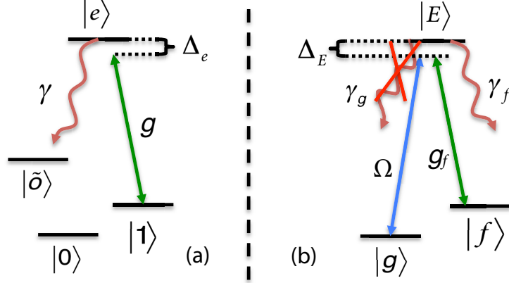
Figure C.1: (a) Level structure of the qubit atoms. Only state |1\rangle couples to the cavity and we assume that the excited level decays to some level |\tilde{0}\rangle , possible identical to |f\rangle or |0\rangle . (b) Level structure of the auxiliary atom and the transitions driven by the weak laser ( \Omega ) and the cavity ( g_f ). We allow for some decay from |E\rangle \rightarrow |g\rangle with decay rate \gamma_g .
