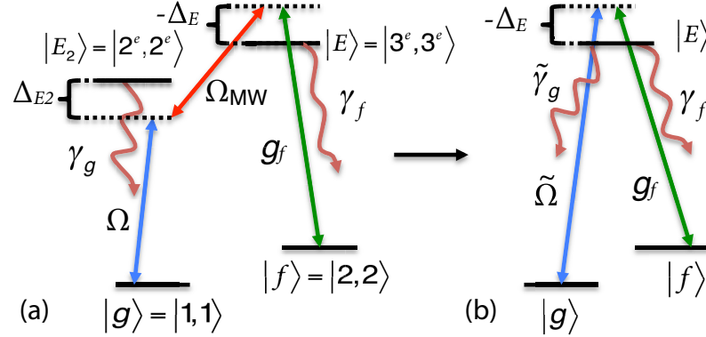
Figure C.3: (a) Level structure of the auxiliary atom and the transitions driven by a weak laser ( \Omega ), a microwave field ( \Omega_{MW} ) and the cavity ( g_f ). We assume that |E\rangle \leftrightarrow |f\rangle is a closed transition and for simplicity we also assume that |E_2\rangle \leftrightarrow |g\rangle is a closed transition but this is not a necessity. The figure also indicates how the levels could be realized in ^{87}\text{Rb} . Here |r^{(e)}, m_F^{(e)}\rangle with r = 1, 2, 3 refers to state |F^{(e)} = r, m_F^{(e)} = r\rangle in 5^2S_{1/2} ( 5^2P_{3/2} ). (b) Effective three level atom realized by mapping the two-photon drive to an effective decay rate \tilde{\gamma}_g and an effective drive \tilde{\Omega}
