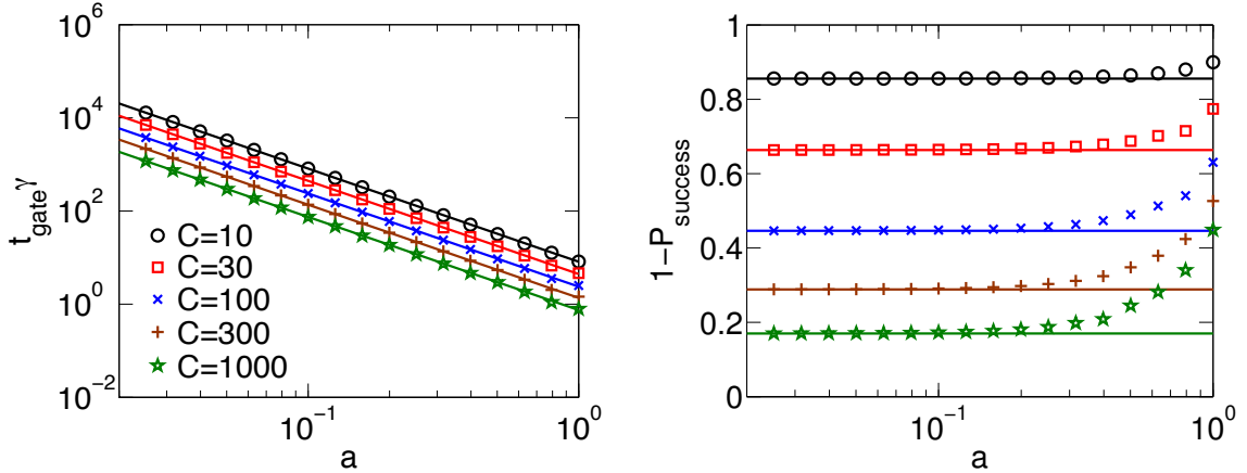
Figure C.4: Gate time (left) and failure probability (right) as a function of driving strength ( a ) for \gamma/\kappa = 0.01 , \gamma_g = 0 , and C \in \{10, 30, 100, 300, 1000\} . The driving strength was assumed to be \Omega = a\gamma\sqrt{C} .
