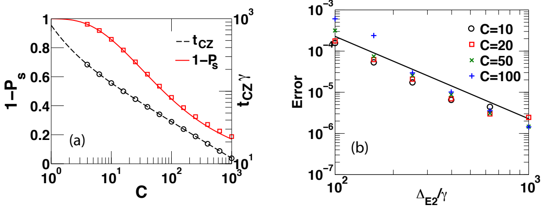
Figure 4.2: (a) Failure probability ( 1 - P_s - left axis) and gate time ( t_{CZ} - right axis) as a function of the cooperativity ( C ) for the CZ gate. The gate time is in units of the inverse linewidth 1/\gamma of the qubit atoms. We have assumed a driving of \Omega = \sqrt{C}\gamma/4 . (b) Gate error as a function of the detuning \Delta_{E2} in the two-photon-driven CZ-gate for C = 10, 20, 50 , and 100 . We have assumed that \Omega_{MW} = 4\gamma C^{1/4} and that \gamma_g = \gamma . The gate error decreases as \gamma^2/\Delta_{E2}^2 and is independent of C . We have assumed \Omega \sim \Delta_{E2}/8 resulting in a gate time \sim 400/\gamma . Solid/dashed lines are analytical results and symbols are numerical simulations (see Appendix C). For both plots, we have assumed \kappa = 100\gamma .
