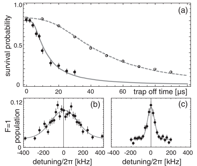
FIG. 2. (a) Release-and-recapture temperature measurement. The closed and open circles show measurements before and after radial cooling, respectively. A Monte Carlo model yields kinetic energies K such that 2K/k_B = 52(4) \mu\text{K} before cooling, and (2K_r/k_B, 2K_a/k_B) = [2.4(1), 158(14)] \mu\text{K} after cooling. (b), (c) Doppler measurement of the axial kinetic energy before and after cooling the axial mode. (b) After radial cooling only, 2K_a/k_B = 129(19) \mu\text{K} . (c) After radial and axial cooling, 2K_a/k_B = 8.1(1) \mu\text{K} .
